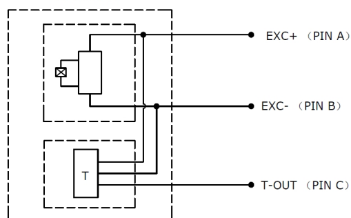
ACCELEROMETER HOUSING
